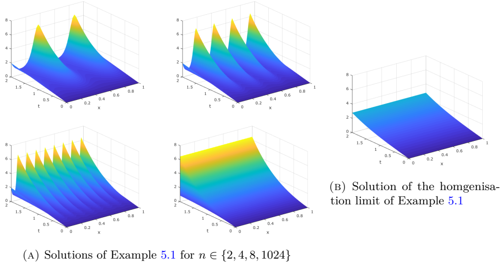
FIGURE 2. Solutions of Example 5.1 for n \in \{2, 4, 8, 1024\} and for the homogenised problem
