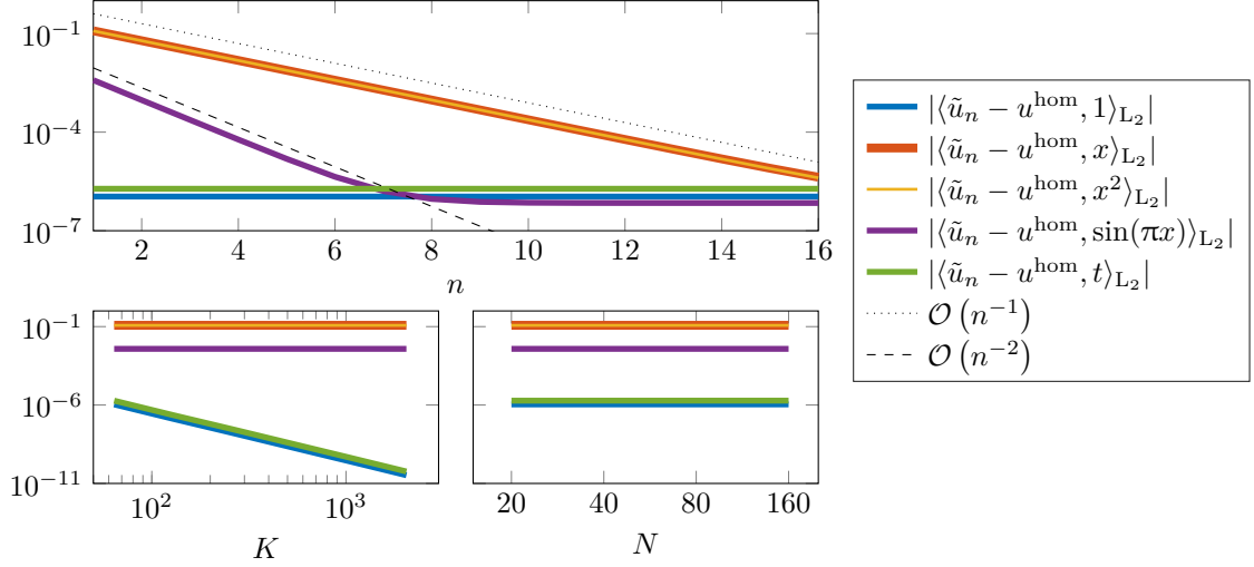
FIGURE 3. Results investigating weak convergence for Example 5.1
