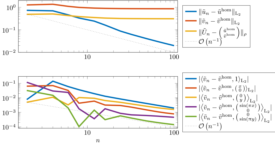
FIGURE 9. Results investigating convergence for Example 5.3 (iii) and (21)
