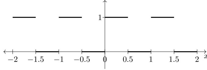
FIGURE 1. Graph of \mathbb{1}_{O_n} for n = 1
