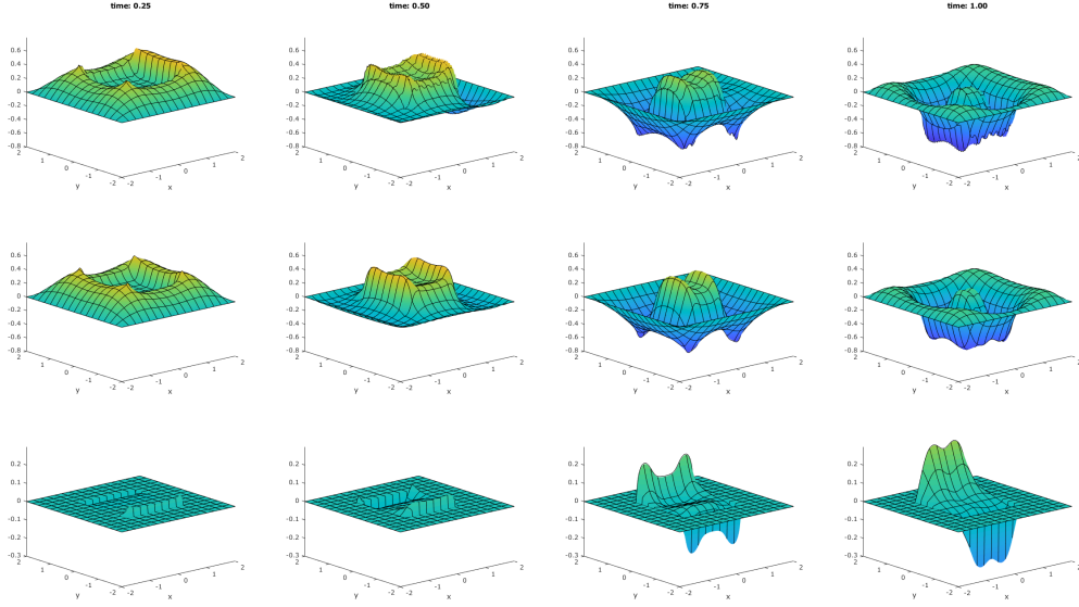
FIGURE 8. Plots of the first component of the solution U_8 of Example 5.3 (iii) (top), the first (middle) and third component (bottom) of \hat{U}^{\text{hom}} of (21) for t \in \{0.25, 0.5, 0.75, 1.0\} (left to right)
