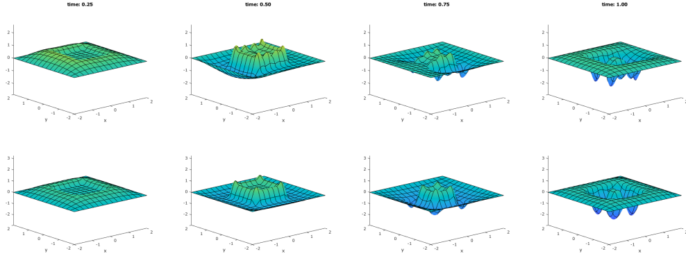
FIGURE 6. Plots of the first component of the solution of Example 5.3 (ii) u_8 (top) and u^{\text{hom}} (bottom) for t \in \{0.25, 0.5, 0.75, 1.0\} (left to right)
