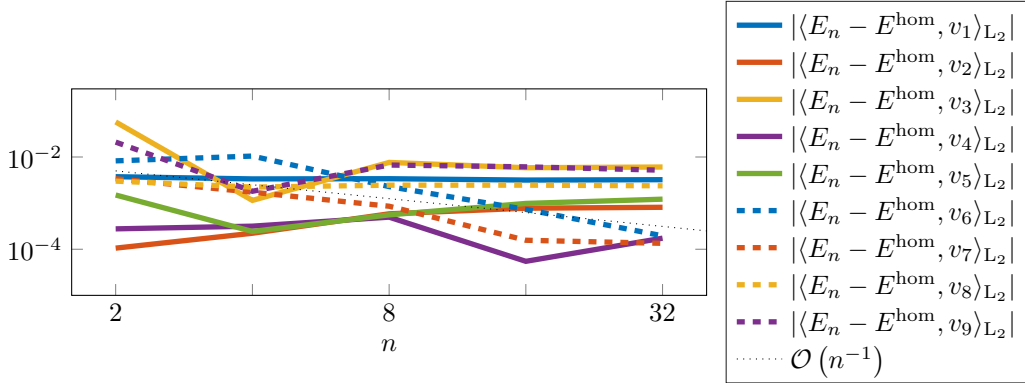
FIGURE 11. Investigation of probable weak convergence of the full 3D Maxwell example (22).
