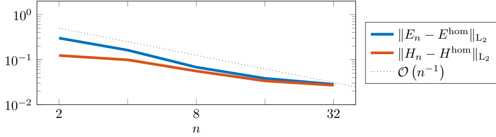
FIGURE 10. Computed errors for the full 3D Maxwell example (22).
